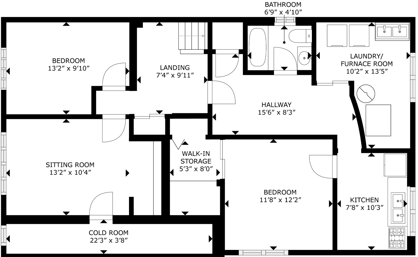
LOWER LEVEL
