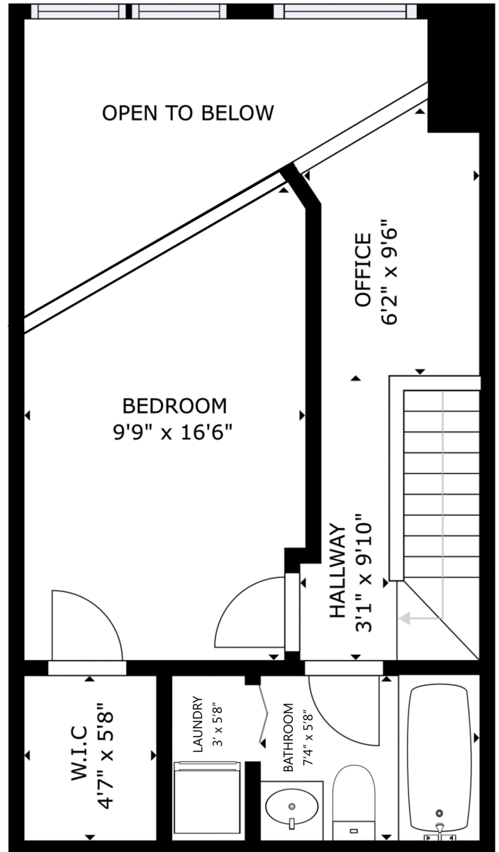
UPPER FLOOR
