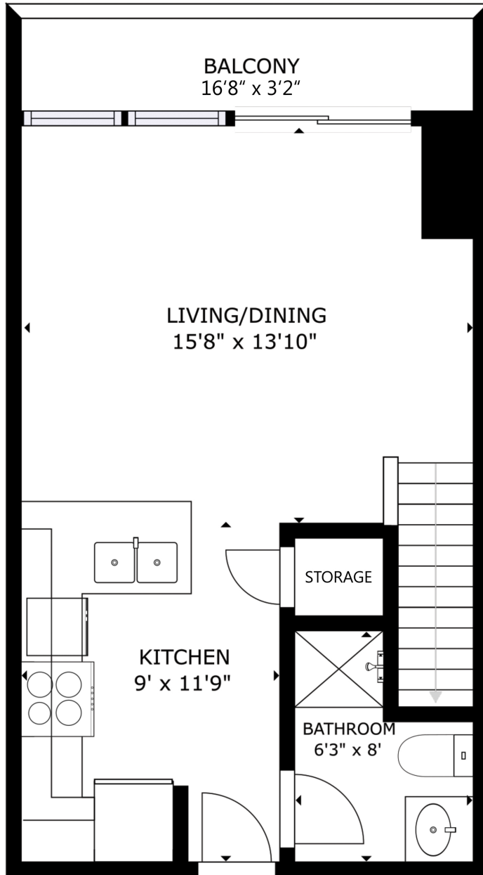
MAIN FLOOR
